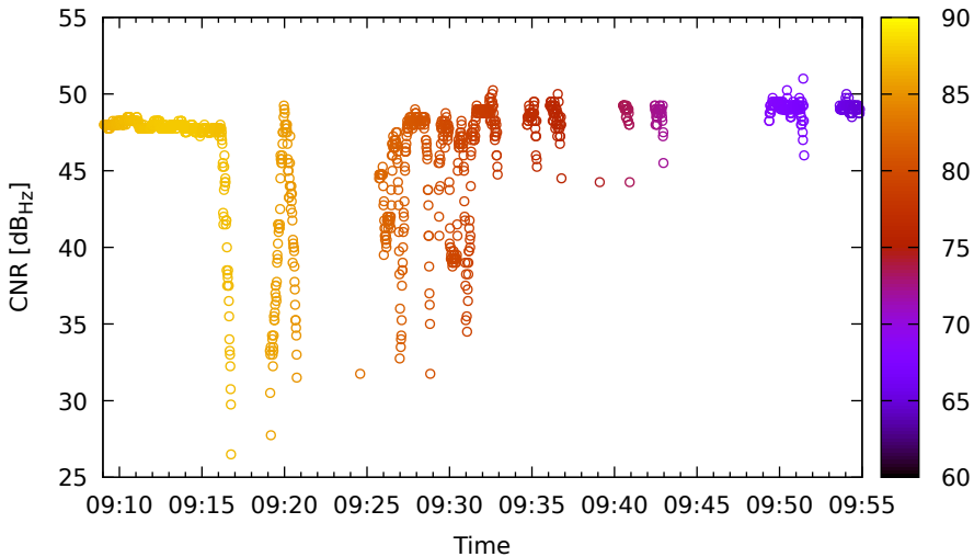
Timeline for R23 (G1) on LeicaGS18 - DOY 262
