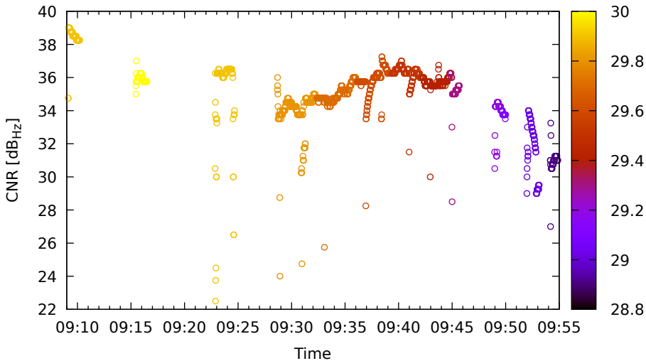
Timeline for C06 (B1) on Xiaomi11T - DOY 262
