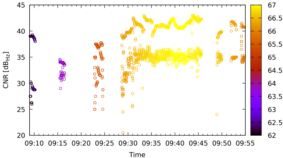
Timeline for C28 (B1) on Xiaomi11T - DOY 262
