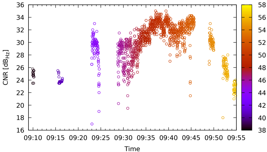
Timeline for E05 (E5a) on Xiaomi11T - DOY 262
