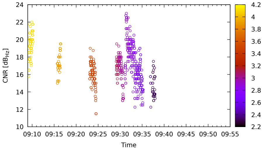
Timeline for E27 (E5a) on Xiaomi11T - DOY 262
