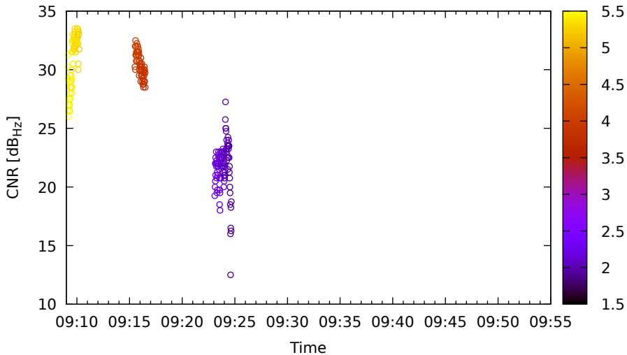
Timeline for E30 (E5a) on Xiaomi11T - DOY 262
