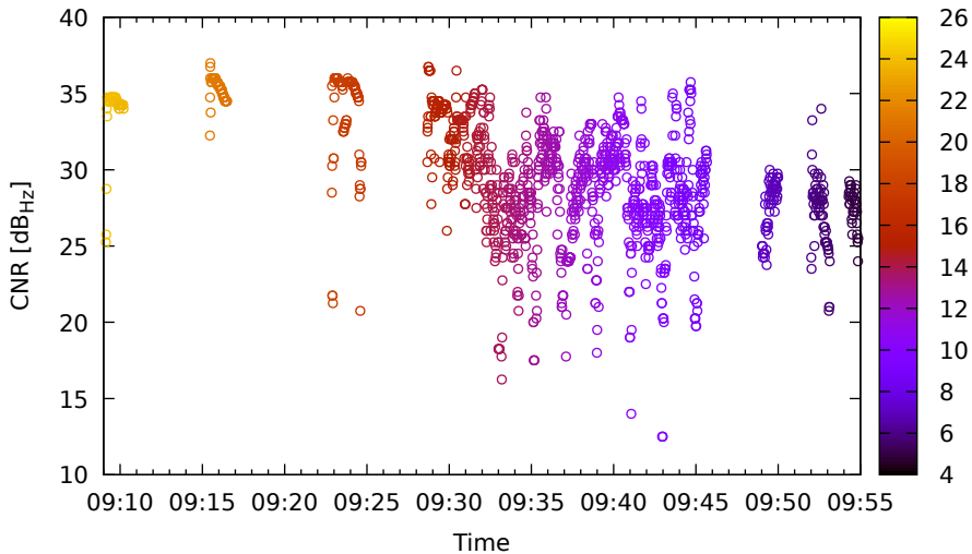
Timeline for G08 (L1) on Xiaomi11T - DOY 262
