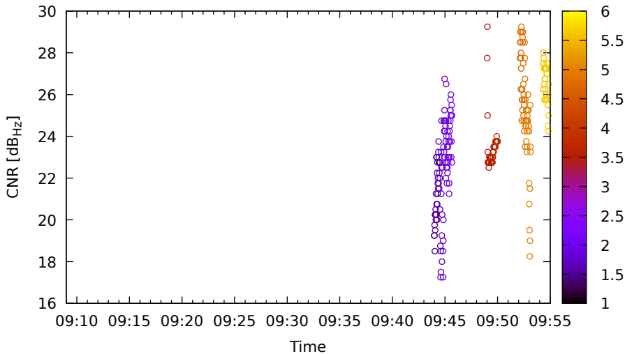
Timeline for G09 (L5) on Xiaomi11T - DOY 262
