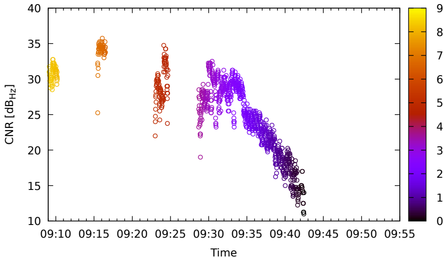
Timeline for G14 (L5) on Xiaomi11T - DOY 262
