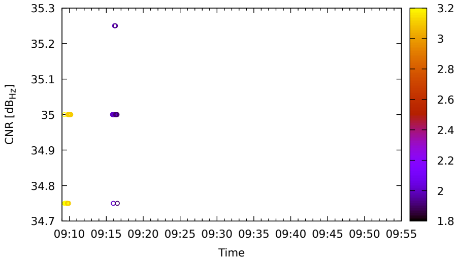
Timeline for R15 (G1) on Xiaomi11T - DOY 262
