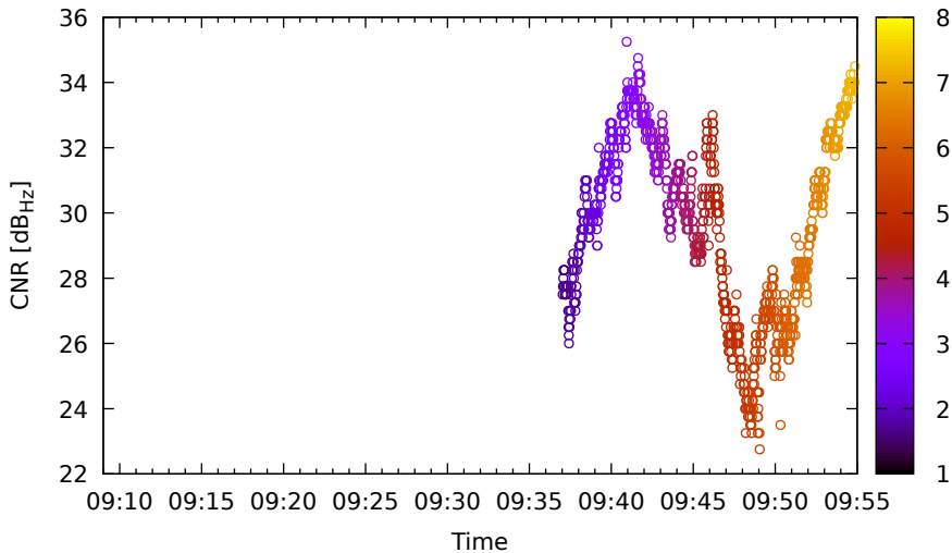
Timeline for E03 (E5a) on XiaomiMi8 - DOY 262
