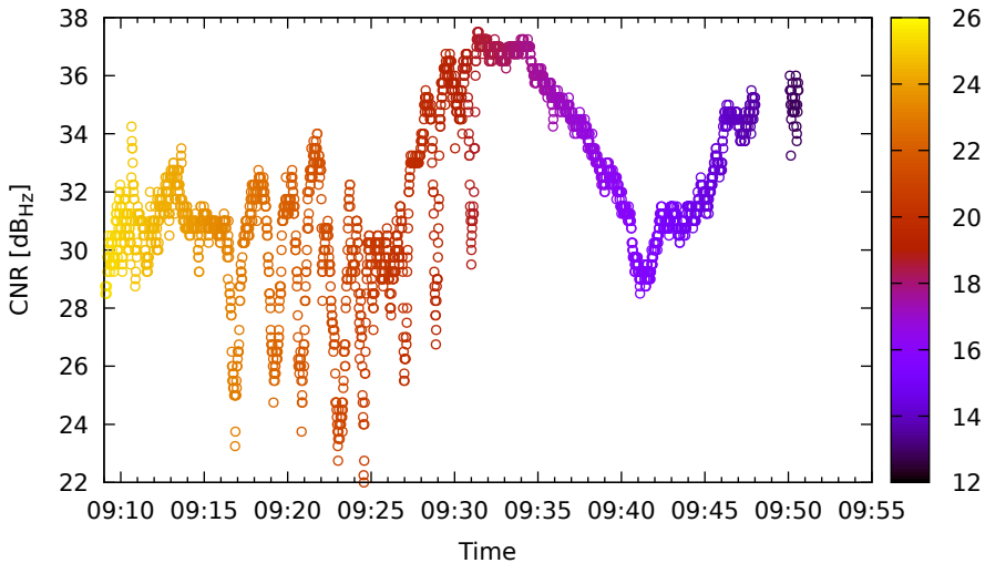
Timeline for E04 (E5a) on XiaomiMi8 - DOY 262
