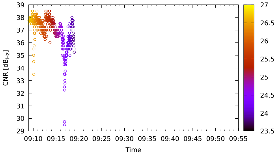
Timeline for E11 (E1) on XiaomiMi8 - DOY 262
