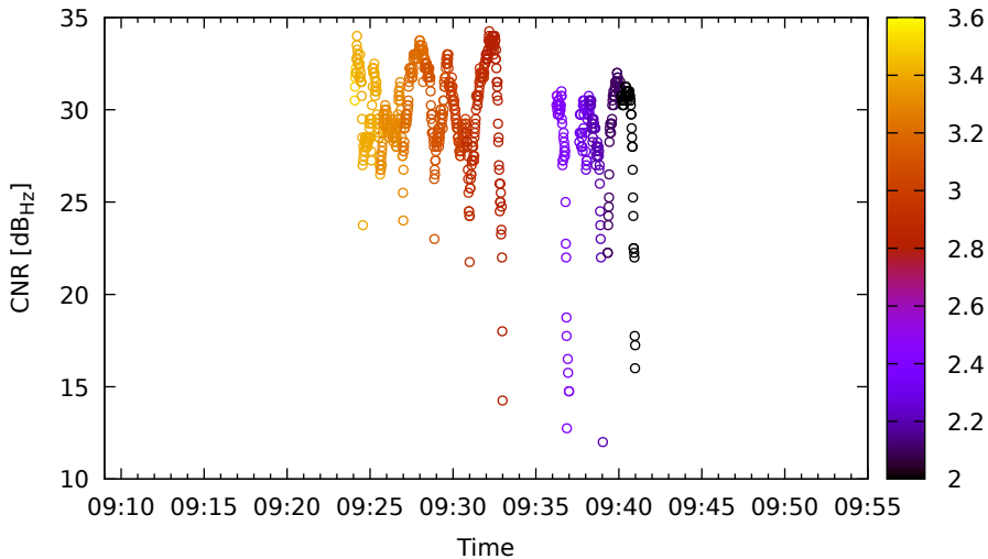
Timeline for E27 (E1) on XiaomiMi8 - DOY 262
