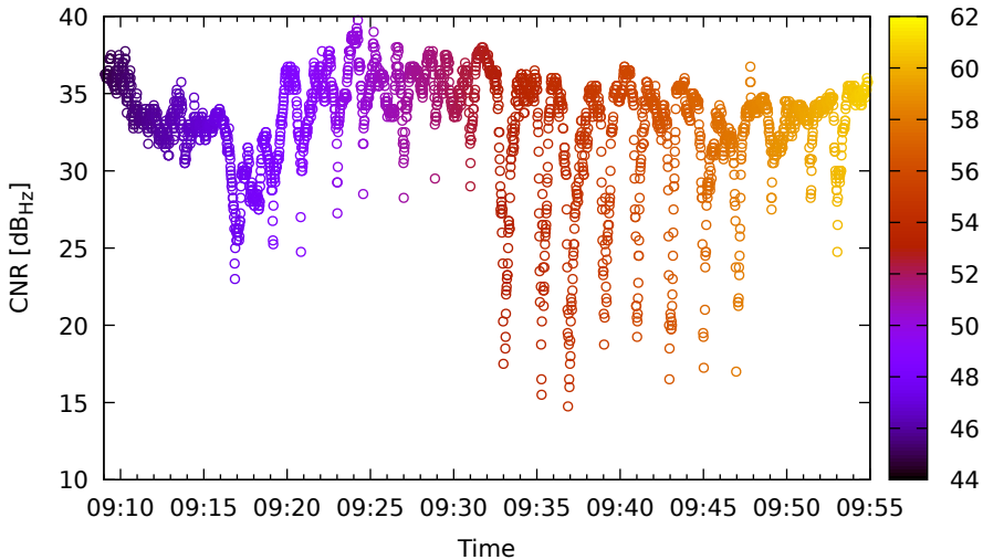
Timeline for E34 (E1) on XiaomiMi8 - DOY 262
