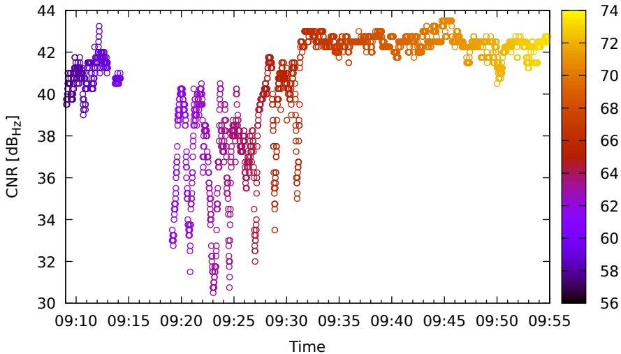
Timeline for G03 (L5) on XiaomiMi8 - DOY 262
