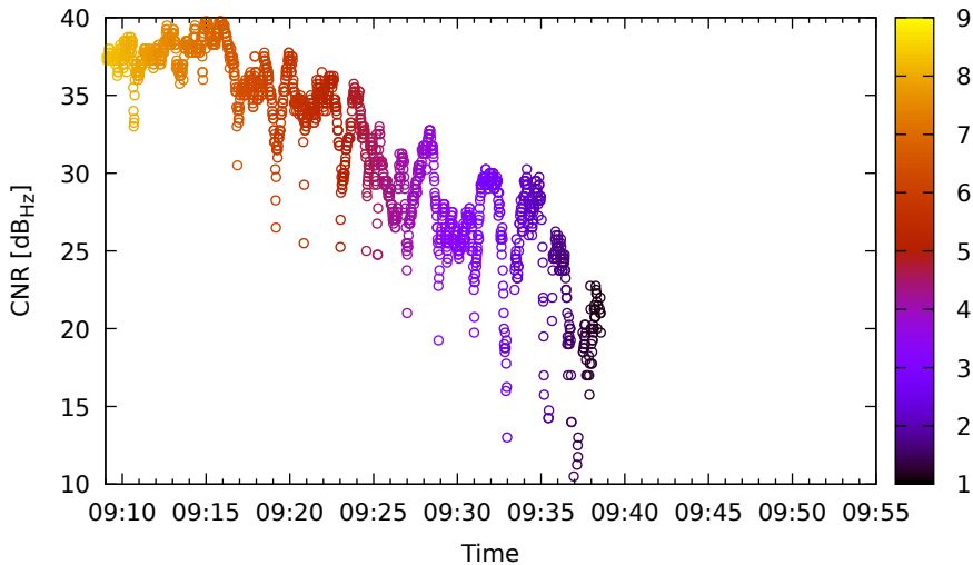
Timeline for G14 (L1) on XiaomiMi8 - DOY 262
