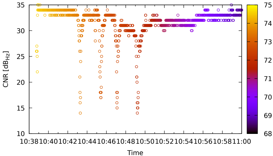
Timeline for G03 (L5) on HuaweiP40 - DOY 262
