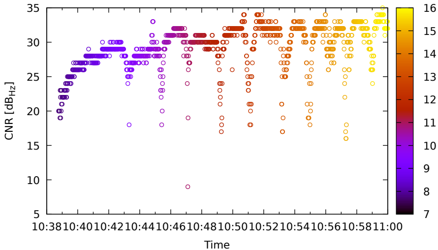
Timeline for G06 (G1) on HuaweiP40 - DOY 262
