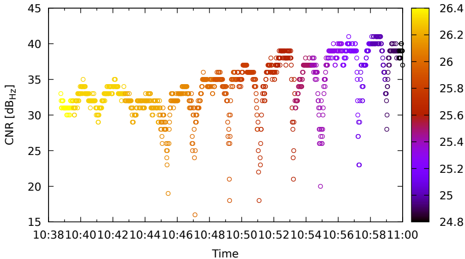
Timeline for G31 (G1) on HuaweiP40 - DOY 262
