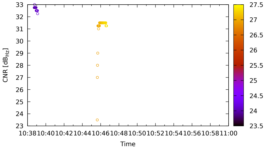
Timeline for G09 (L5) on Xiaomi11T - DOY 262
