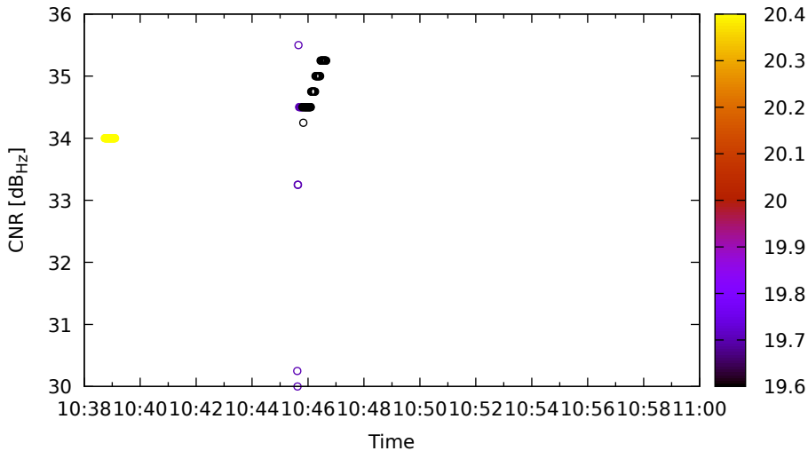
Timeline for C16 (B1) on XiaomiMi8 - DOY 262
