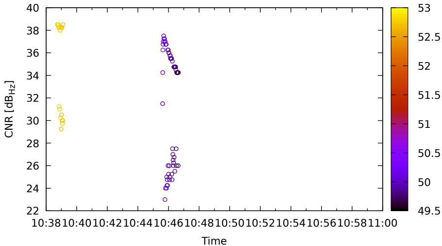
Timeline for C28 (B1) on XiaomiMi8 - DOY 262
