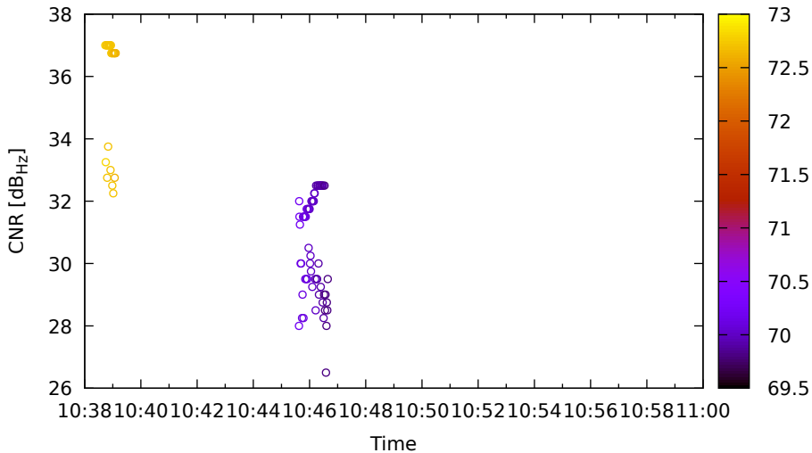
Timeline for C33 (B1) on XiaomiMi8 - DOY 262
