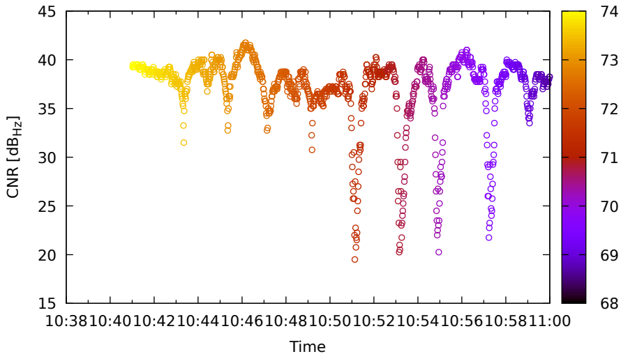
Timeline for G03 (L1) on XiaomiMi8 - DOY 262
