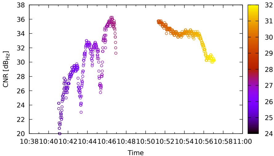
Timeline for G09 (L5) on XiaomiMi8 - DOY 262
