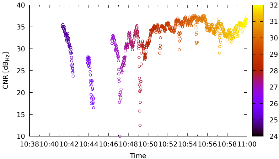
Timeline for R02 (G1) on XiaomiMi8 - DOY 262
