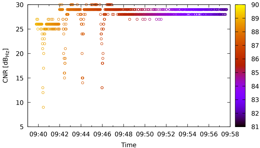
Timeline for E12 (E1) on HuaweiP40 - DOY 263
