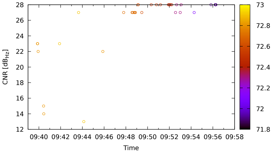
Timeline for E19 (E5a) on HuaweiP40 - DOY 263
