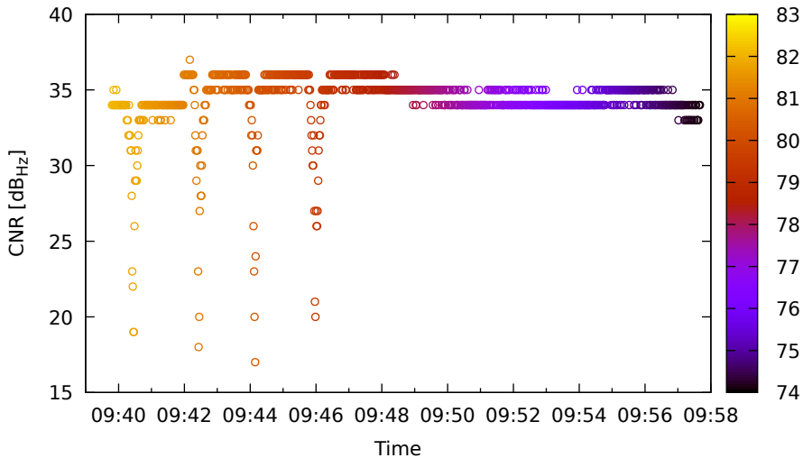
Timeline for G01 (L5) on HuaweiP40 - DOY 263
