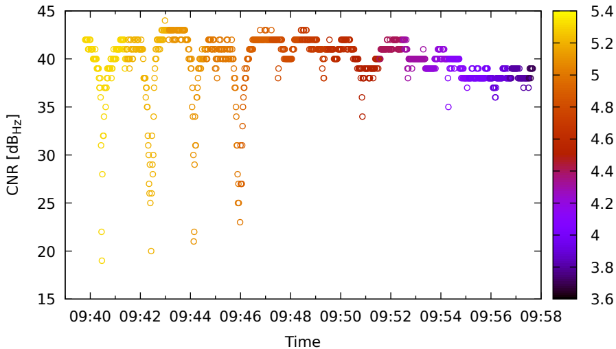
Timeline for R09 (G1) on HuaweiP40 - DOY 263
