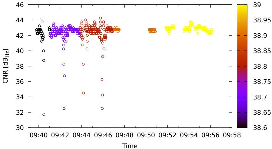
Timeline for C09 (B3) on LeicaGS18 - DOY 263
