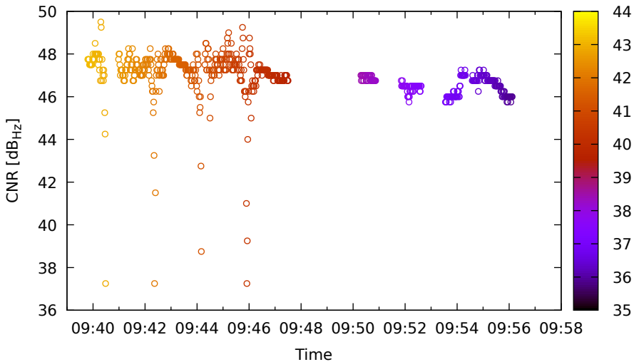
Timeline for C34 (B3) on LeicaGS18 - DOY 263
