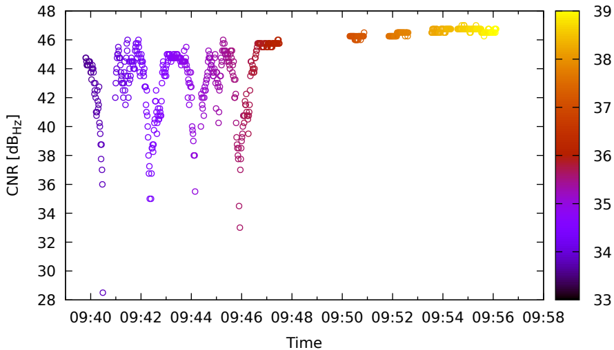
Timeline for E11 (E5a) on LeicaGS18 - DOY 263
