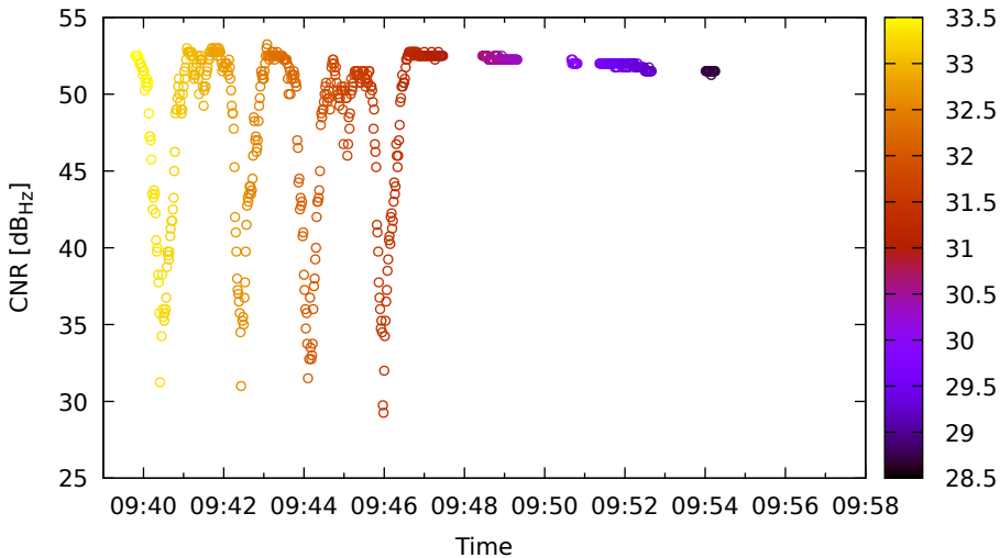
Timeline for E33 (E5) on LeicaGS18 - DOY 263
