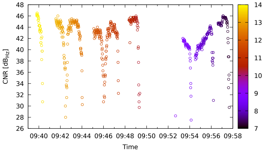
Timeline for G32 (L1) on LeicaGS18 - DOY 263
