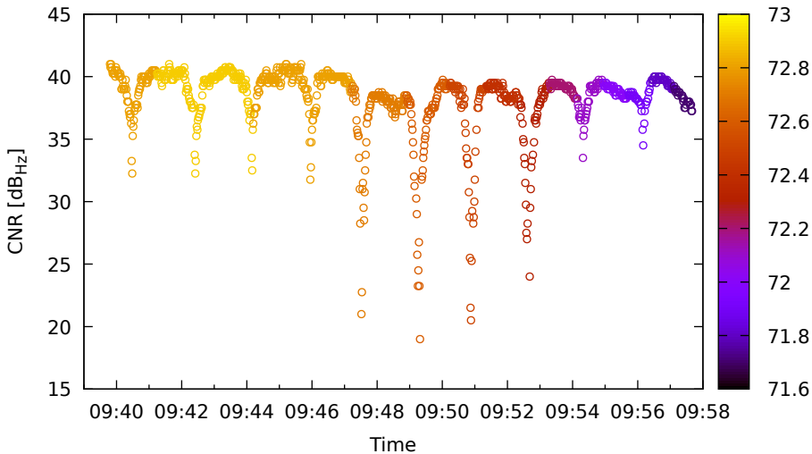
Timeline for E19 (E1) on SamsungS20 - DOY 263
