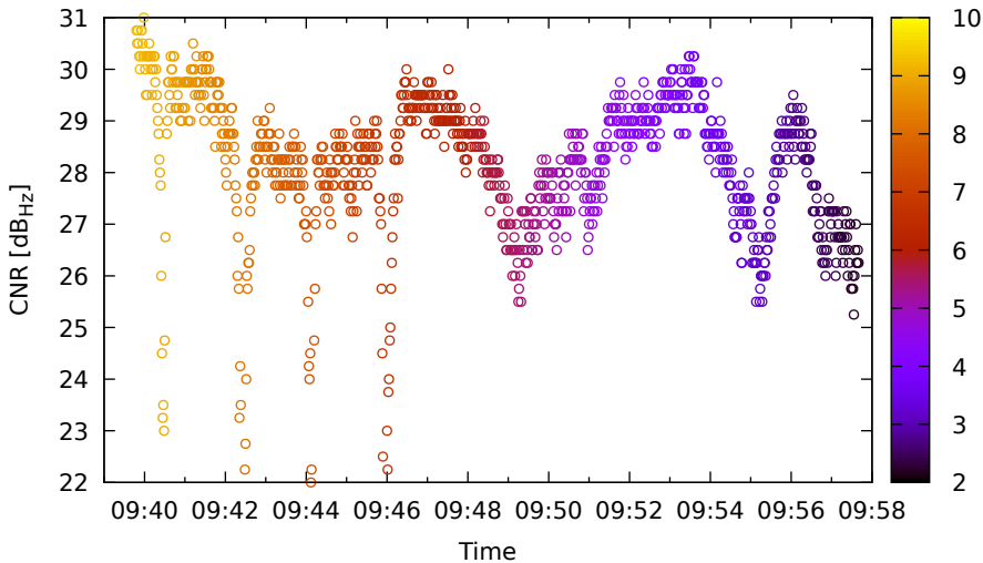
Timeline for G08 (L5) on SamsungS20 - DOY 263
