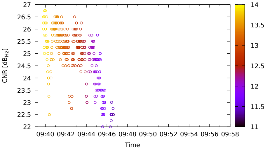
Timeline for G32 (L5) on SamsungS20 - DOY 263
