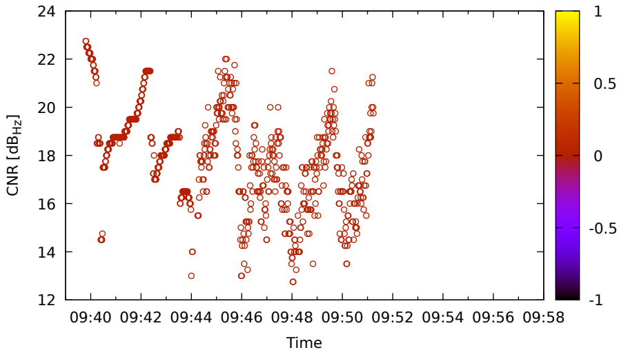
Timeline for E02 (E5a) on Xiaomi11T - DOY 263
