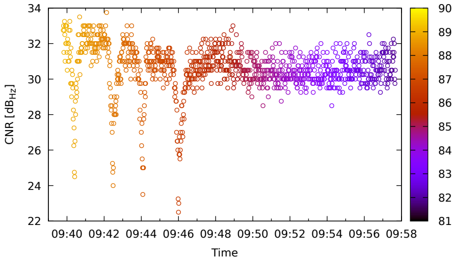
Timeline for E12 (E5a) on Xiaomi11T - DOY 263
