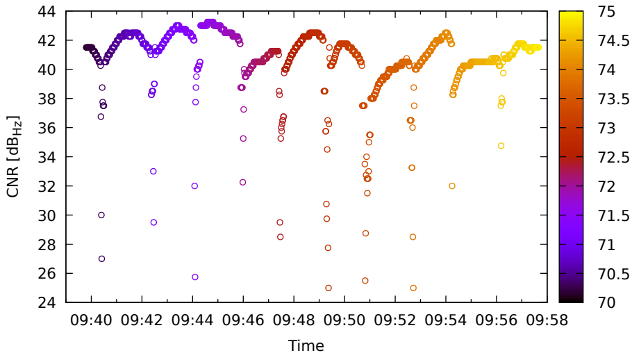
Timeline for G03 (L1) on Xiaomi11T - DOY 263
