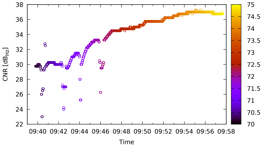
Timeline for G03 (L5) on Xiaomi11T - DOY 263
