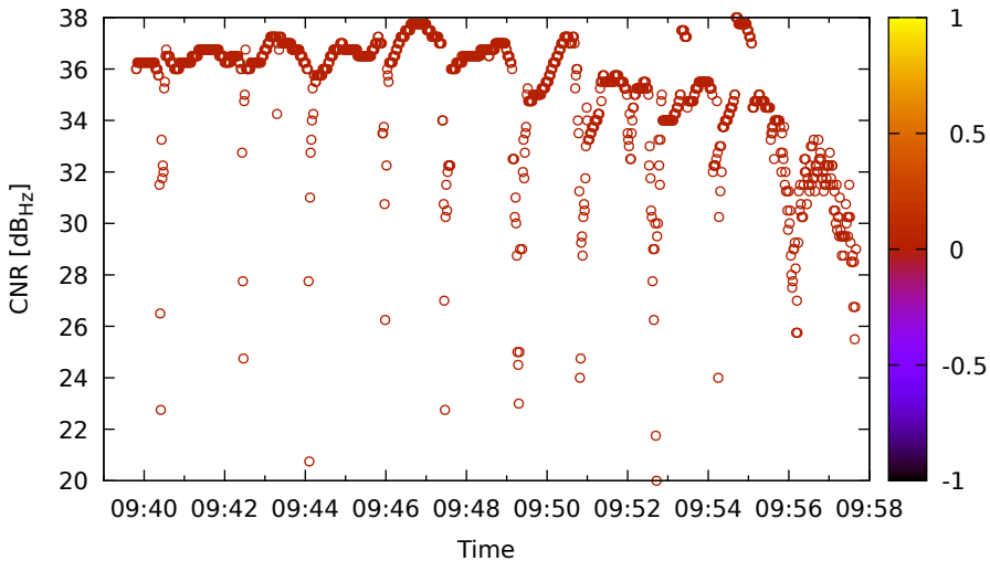
Timeline for G28 (L1) on Xiaomi11T - DOY 263
