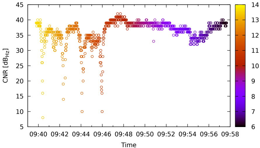
Timeline for R08 (G1) on Xiaomi11T - DOY 263
