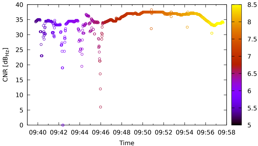
Timeline for R10 (G1) on Xiaomi11T - DOY 263
