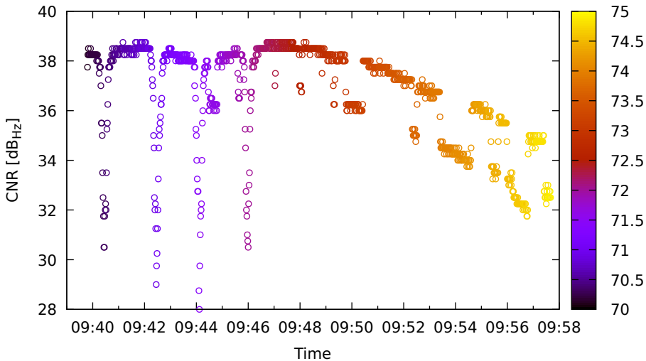
Timeline for G03 (L5) on XiaomiMi8 - DOY 263
