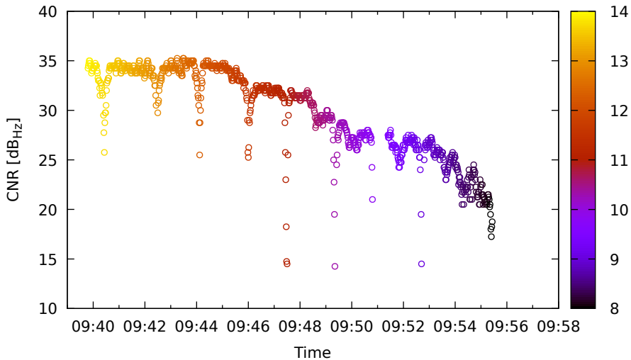
Timeline for G32 (L1) on XiaomiMi8 - DOY 263
