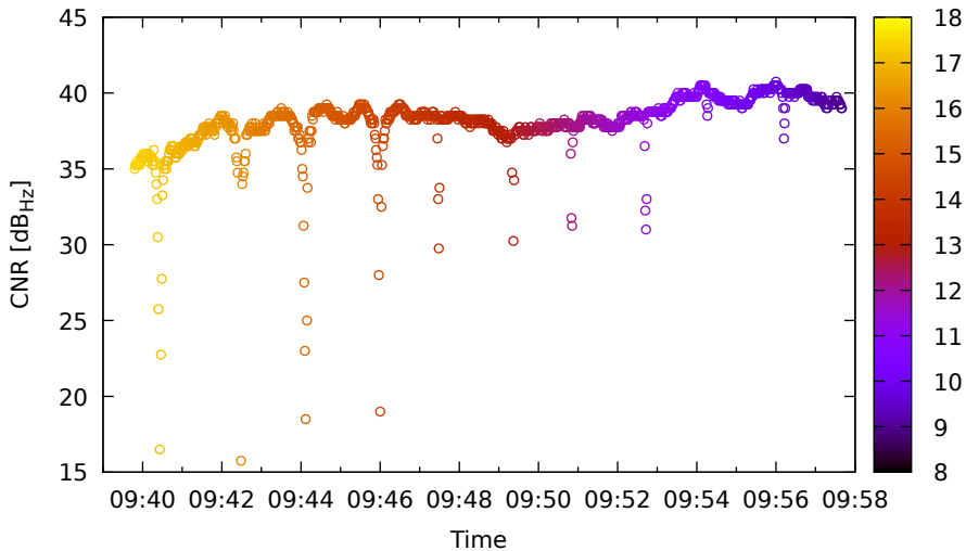
Timeline for R23 (G1) on XiaomiMi8 - DOY 263
