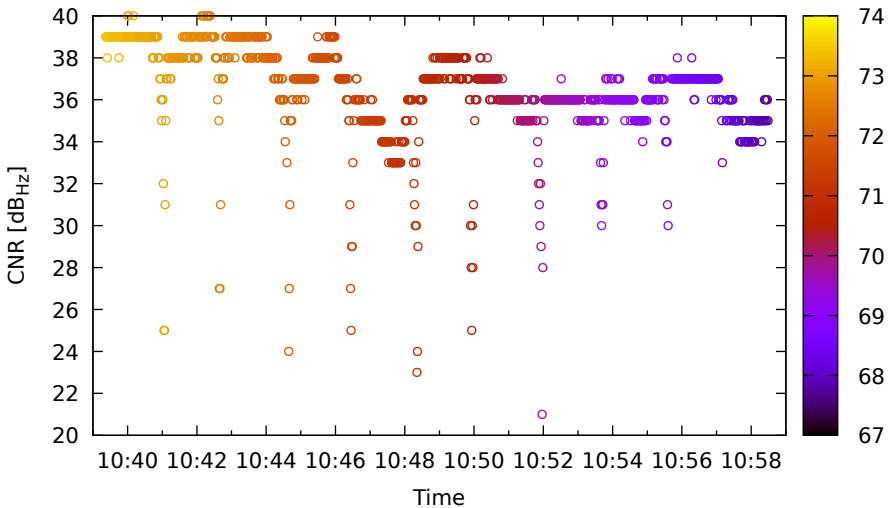
Timeline for G03 (L1) on HuaweiP40 - DOY 263
